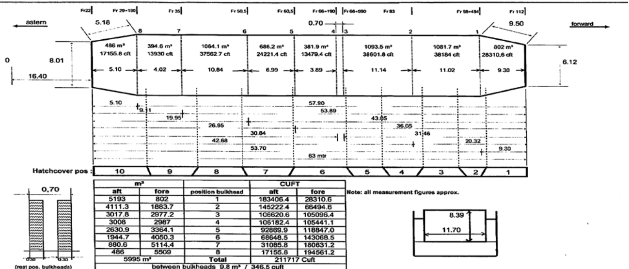
m.v. CELTIC FREEDOM Hold Dimensions & Bulkhead Positions
